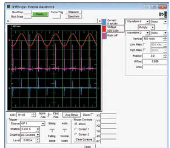
Power Analyzer oscilloscope panel
